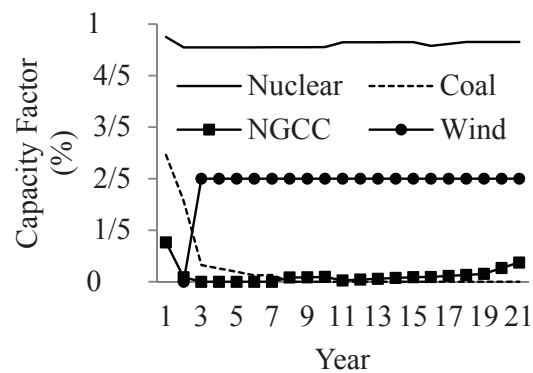
Figure 5 Capacity Factors
