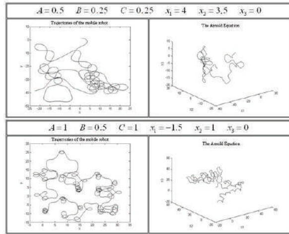
Figure 10 Robot motion is unpredictable and sensitively dependent on initial conditions
