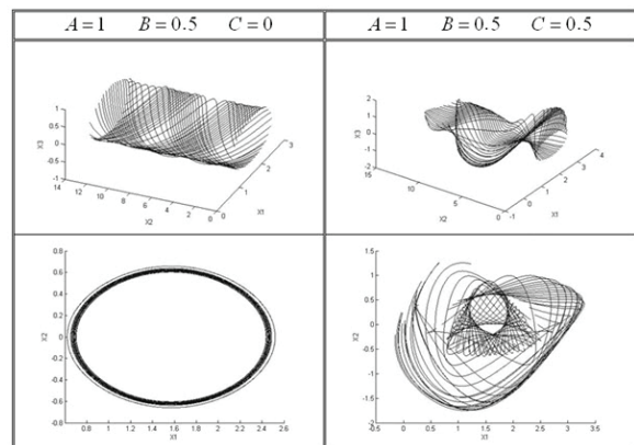
Figure 3 Arnold equation trajectories
