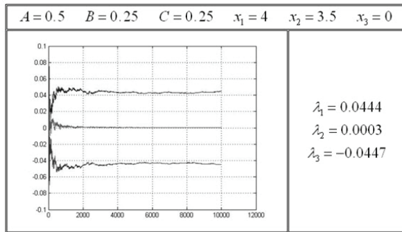
Figure 4 Lyapunov exponent
