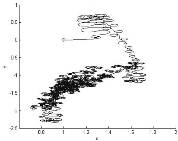
Figure 14 Motion trajectories with different initial conditions
