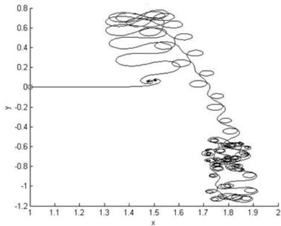
Figure 11 Motion trajectories with Lorenz equation
