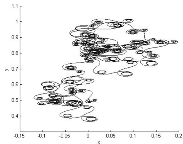
Figure 15 Motion trajectories with different Rayleigh number ( r = 50 )
