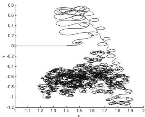
Figure 13 Motion trajectories with 100 time units
