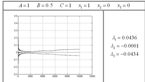
Figure 6 Lyapunov Exponent
