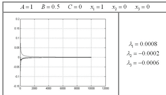
Figure 5 Lyapunov exponent
