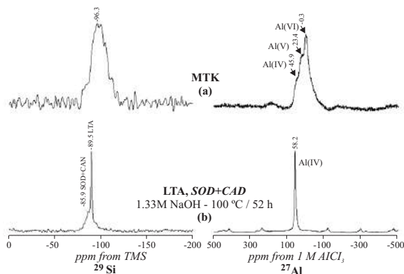
Figure 7 29 Si and 27 Al NMR spectra of the (a) metakaolinite and (b) representative synthesis products obtained after hydrothermal reaction of metakaolinite with NaOH activator agent
