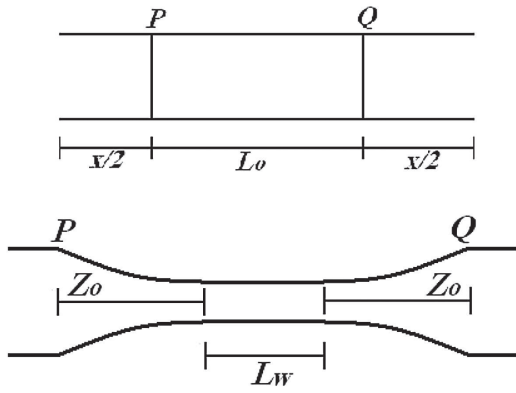
Figure 2 Schematic diagram of an optical fiber taper at time t' and t'+\delta t . PQ has been stretched to form a narrower taper waist
