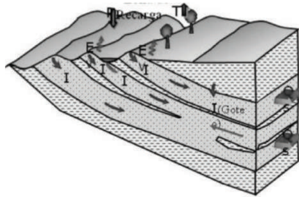
Figure 1 Schematic conceptual model of the Morroa aquifer (Source: Carsucre, scheme not scaled)
