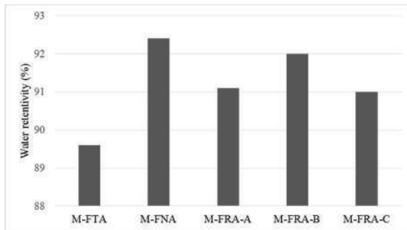
Figure 4 The water retention in mortars made with natural (M-FTA, M-FNA) and recycled (M-FRA-A, M-FRA-B, M-FRA-C) aggregates
