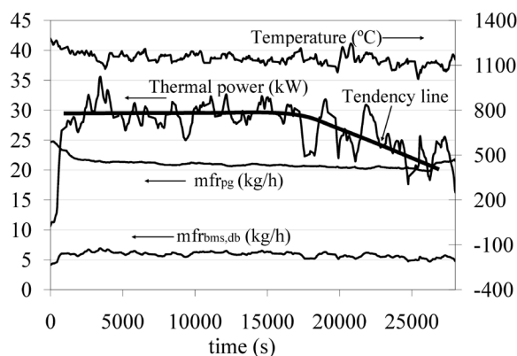
Figure 5 Evolution of temperature, thermal power of producer gas and mass flow rate of producer gas and biomass
