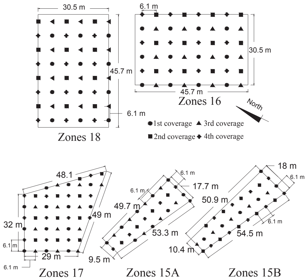
Figure 5 Geometry of the tested zones and distribution of the explosives
