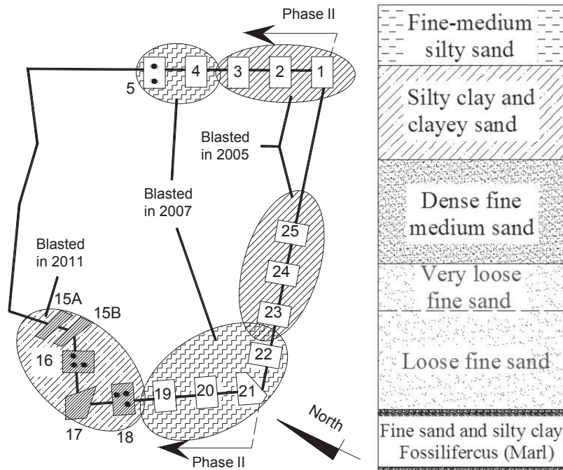
Figure 2 (a) Plain view and blasting sequence of the tested site and (b) soil profile
