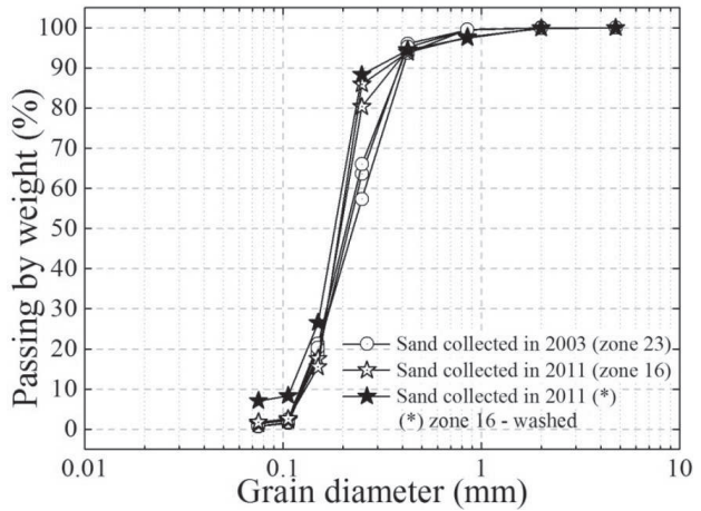
Figure 4 Grain size distribution of the collected sand
