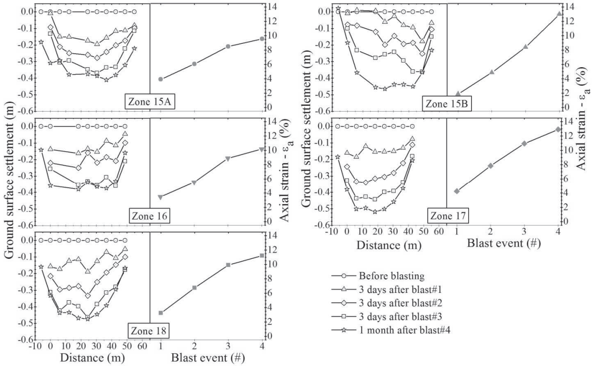
Figure 6 Ground surface settlements measured at the tested zones
