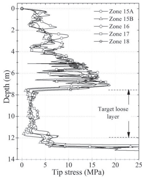
Figure 3 CPT sounding in zones 15A, 15B, 16, 17 and 18
