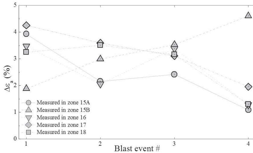
Figure 7 Axial strain increment after each consecutive blast event
