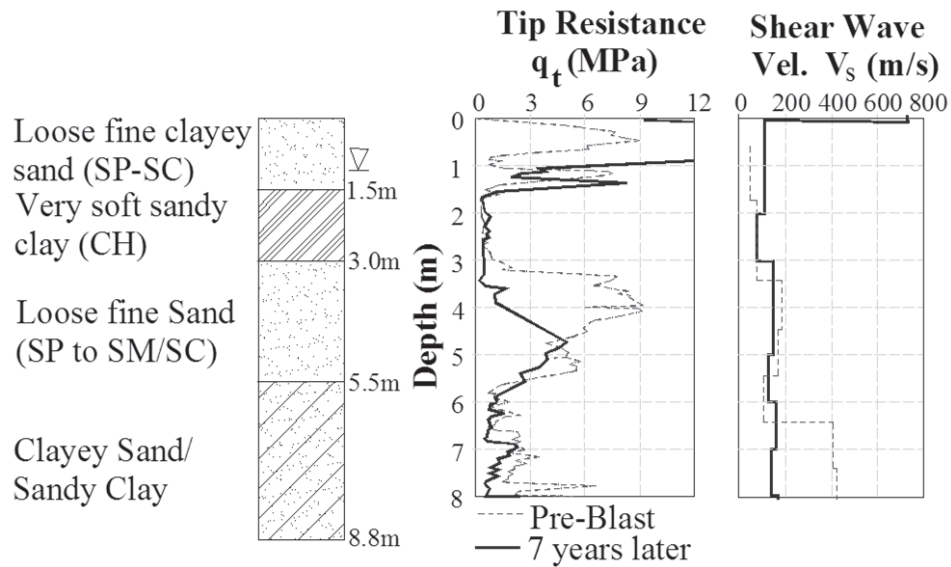
Figure 1 CPT tip resistance and shear wave velocity measurements before and 7 years after blasting. After [4]
