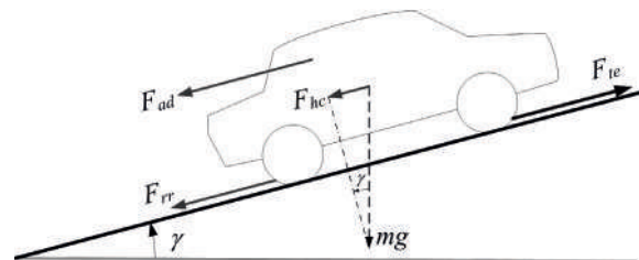
Figure 5 Forces acting on the EV
