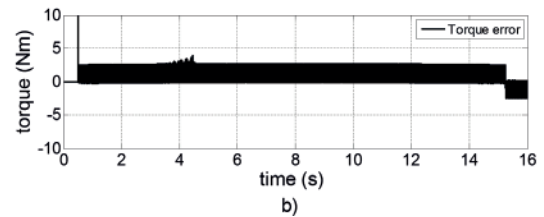
Figure 12 a) Desired vs. estimated torque, b) torque error
