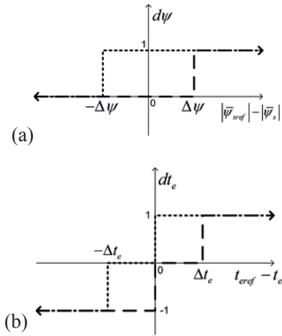
Figure 9 Hysteresis comparators for: a) flux and b) torque
