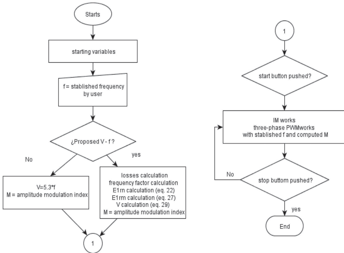
Figure 8 PSoc 5 algorithm
