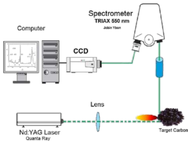
Figure 1 Experimental Setup [9]
