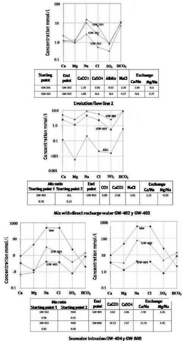
Figure 9 Schoeller diagrams and results of inverse modeling (moles)
