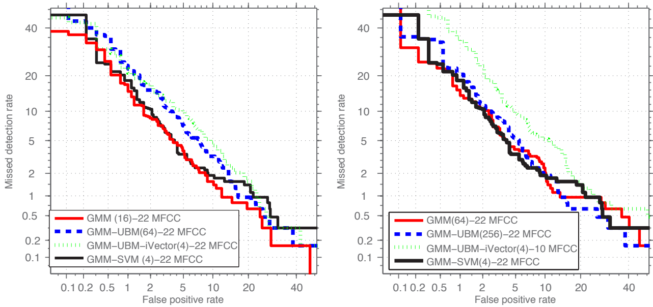
(a) Sex detector using MFCC extracted from speech
