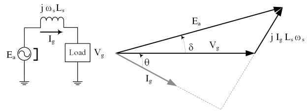
Figure 2 Equivalent circuit and Phasor diagram of a PMSG
