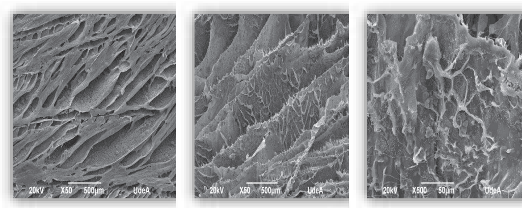
Figure 7 SEM micrographs of CH/BGp/PVA scaffold
