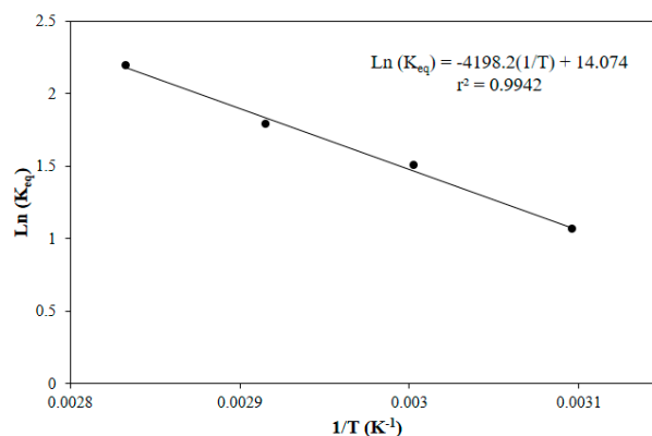
Figure 11 van't Hoff plot for acetic acid esterification with nopol for nopol acetate production
