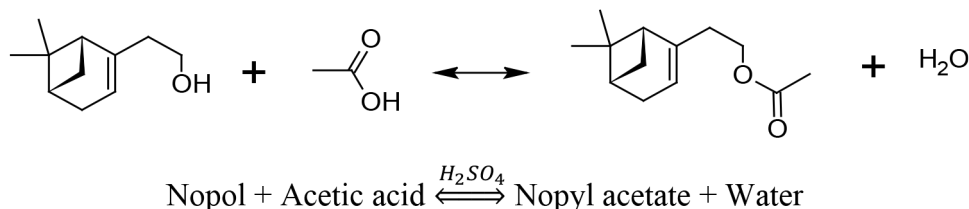
Scheme 2 Synthesis of nopyl acetate ( \text{C}_{13}\text{H}_{20}\text{O}_2 ) starting from nopol ( \text{C}_{11}\text{H}_{18}\text{O} ) and acetic acid ( \text{CH}_3\text{COOH} )
