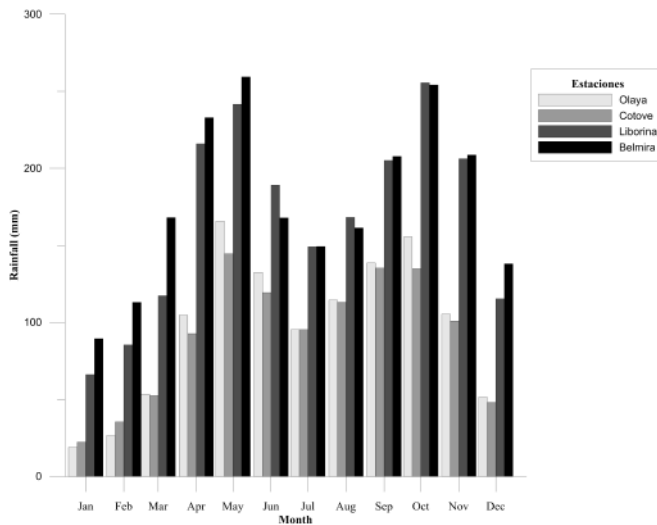
Figure 5 Mean Rainfall Recorded in Weather Stations of the Area
