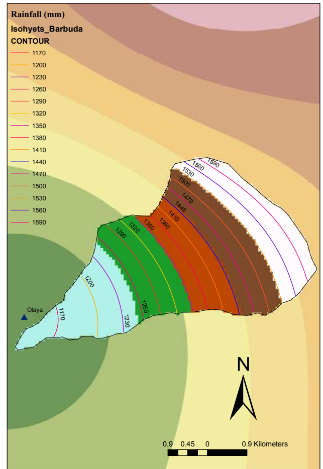
Figure 10 Isohyetal map of the Barbuda stream basin
