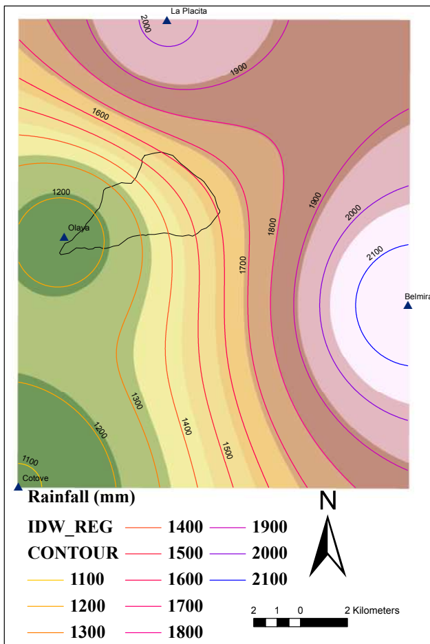
Figure 9 Isohyetal map, region of interest
