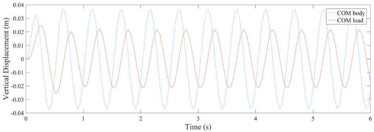
Figure 3 Dynamic response of the model used for M_2 = 25 \text{ kg} , K_2 = 1000 \text{ N/m} and B_2 = 138 \text{ Ns/m}
