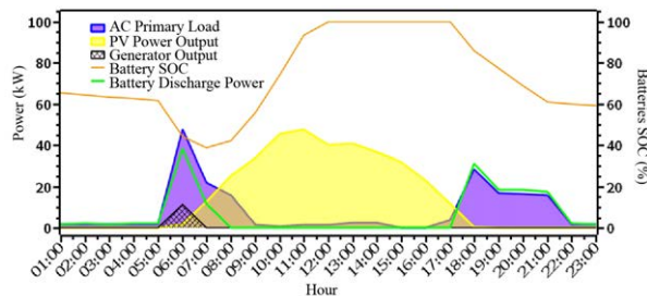
Figure 8 Energy flow of the photovoltaic battery and diesel system to meet the demand
