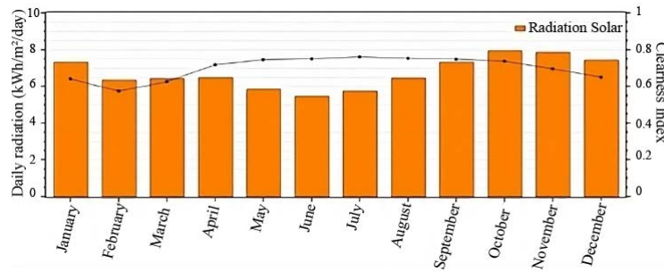
Figure 3 Monthly solar radiation profile and clearness index in the rural community of San Juan de Tarucani
