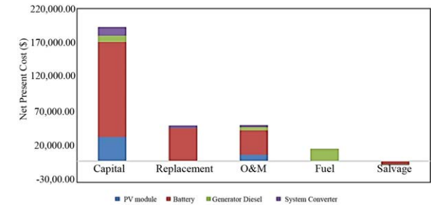
Figure 6 Cash flow from the optimal configuration of the HES
