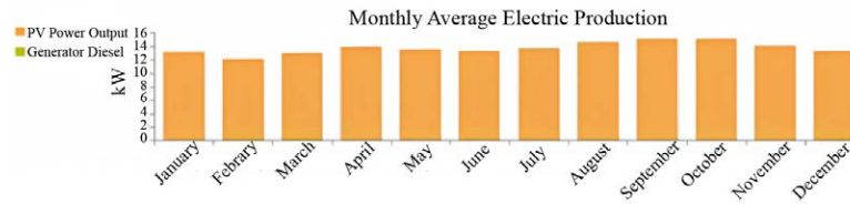
Figure 7 Monthly electricity production from the photovoltaic and generator optimal system
