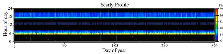
Figure 2 Annual load profile of San Juan de Tarucani community
