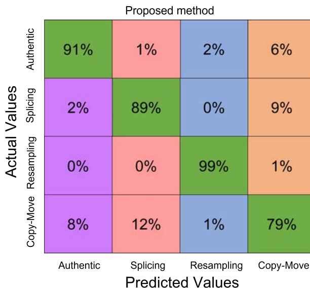
Figure 4 Confusion matrix of the proposed method
