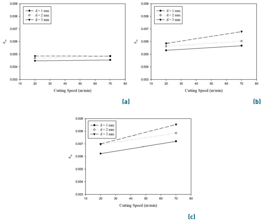
Figure 2 Strain plotted against cutting speed for the turned annealed AISI 1020 steel, with a feed rate of (a) 0.05 mm/rev; (b) 0.15 mm/rev; and (c) 0.25 mm/rev
