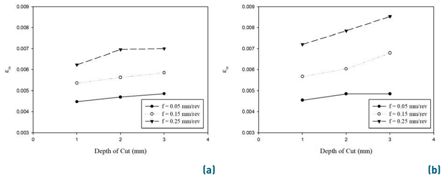
Figure 3 Strain plotted against depth of cut for turned annealed AISI 1020 steel, with a cutting speed of (a) 20 m/min; and (b) 70 m/min
