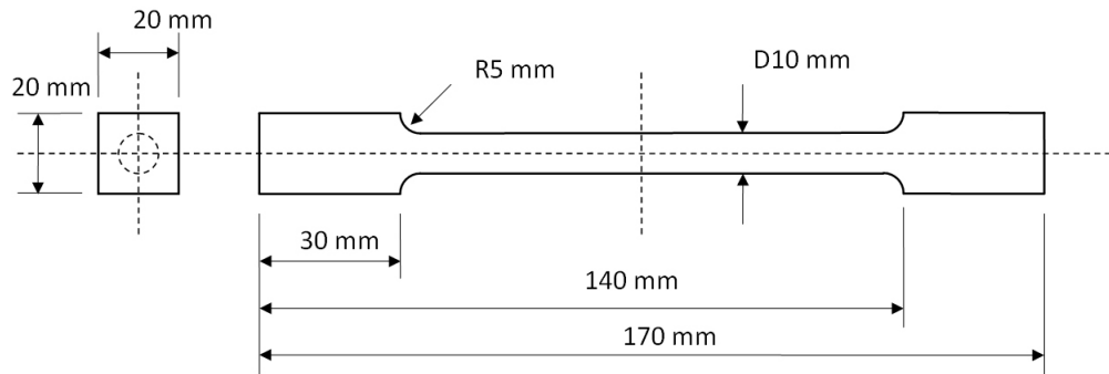
Figure 1 Torsion specimen's dimensions
