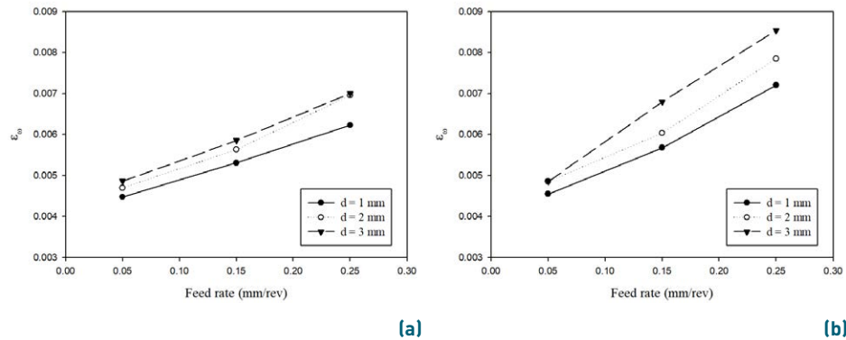
Figure 4 Strain plotted against feed rate for the turned annealed AISI 1020 steel, with a cutting speed of (a) 20 m/min, and (b) 70 m/min
