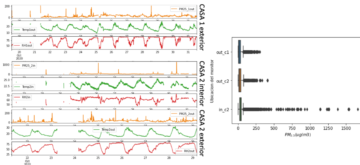
Figure 5 Particulate Matter concentrations, RH and temperature measured (A) Casa 1, (B) Casa2, (C) Box plot figures of PM2.5 concentration distributions in Casa 1 y Casa 2
