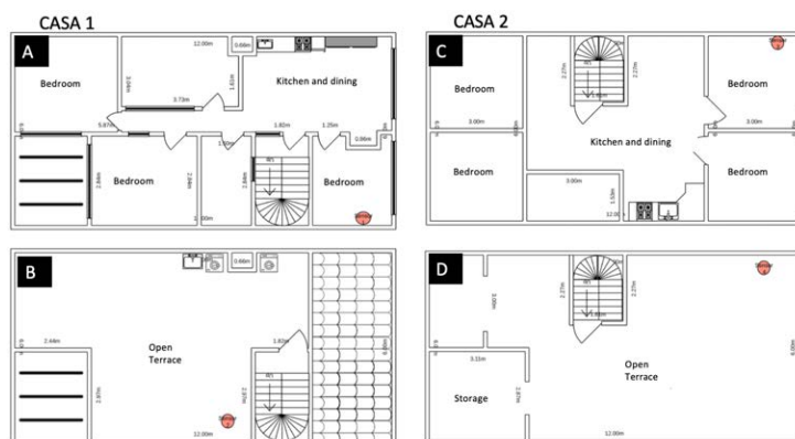
Figure 4 Sensor location (A) Casa 1 interior, (B) House 1 Terrace, (C) Casa 2 interior, (D) House 2 terrace
