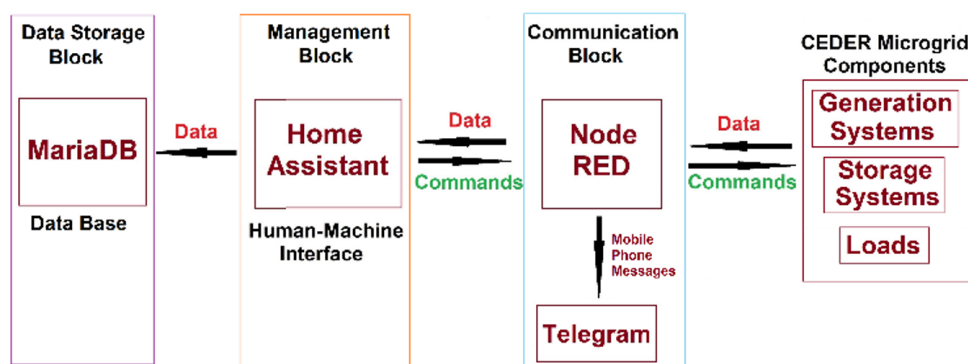
Figure 2 Elements of CEDER microgrid control system [27]
