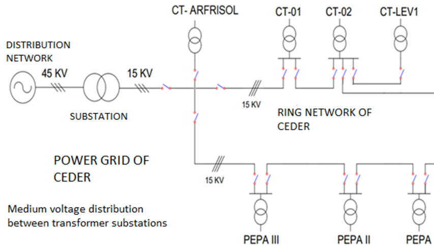
Figure 1 Medium-voltage distribution between transformation centres.
