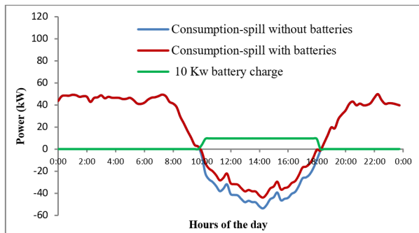
Figure 6 Load study at 10 kW.
