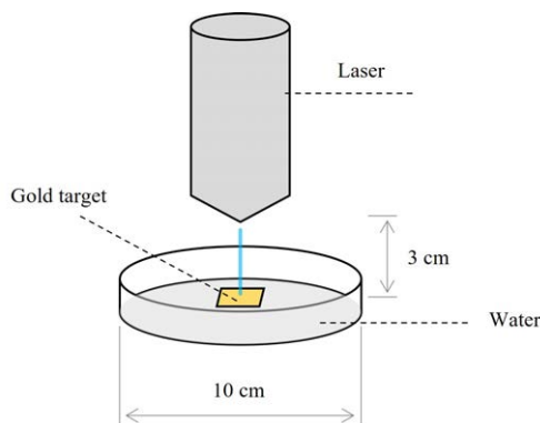
Figure 1 Schematics of the experimental setup
