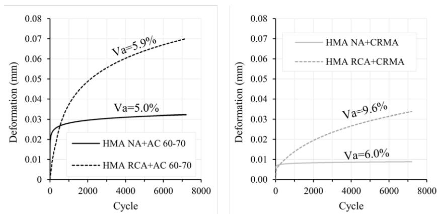
Figure 15 Permanent deformation test at 20 °C
