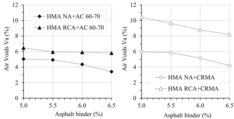
Figure 6 Variation of Va with the conventional and modified asphalt content for mixtures with NA and RCA
