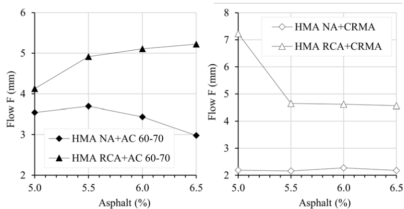
Figure 10 Variation of Marshall Flow with the conventional and modified asphalt content for mixtures with NA and RCA
