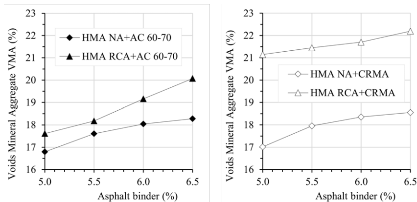
Figure 7 Variation of VMA with the conventional and modified asphalt content for mixtures with NA and RCA
