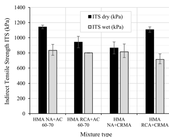
Figure 12 ITS test results
