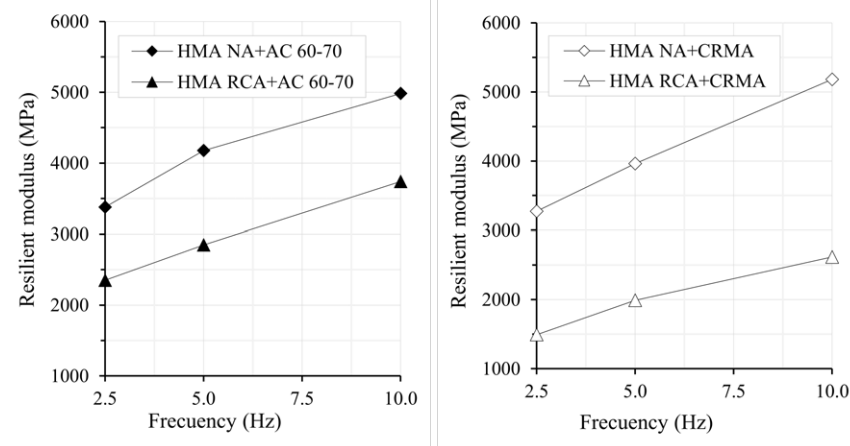
Figure 14 Resilient modulus at 20 °C
