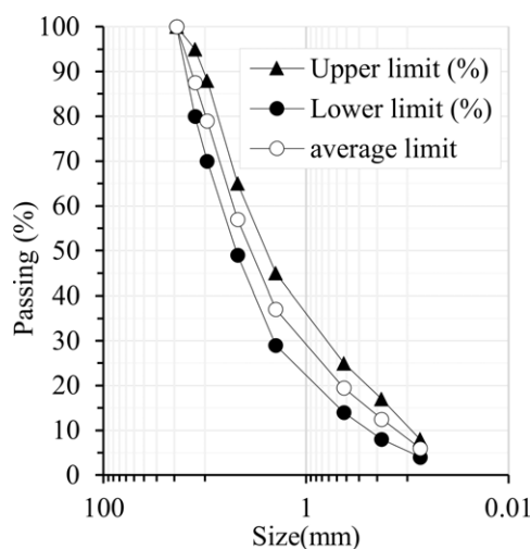
Figure 2 Particle size distribution of HMA
