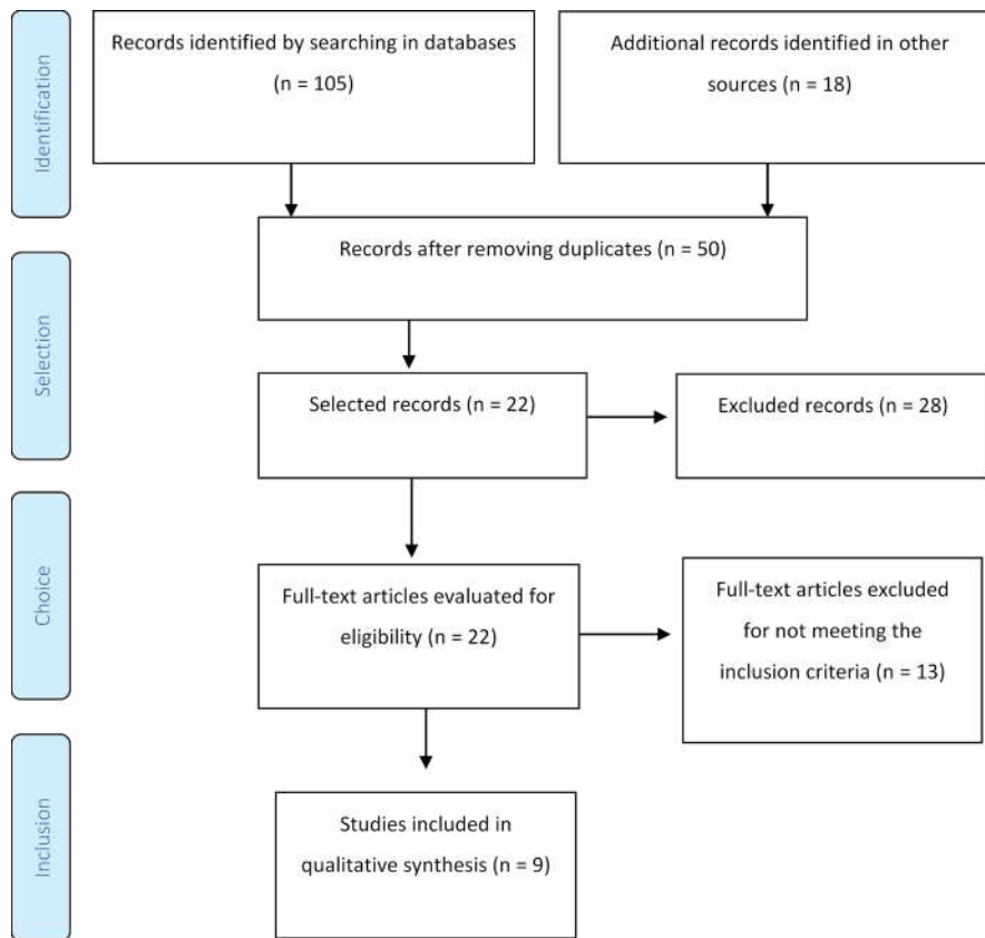
Figure 1. PRISMA flowchart
