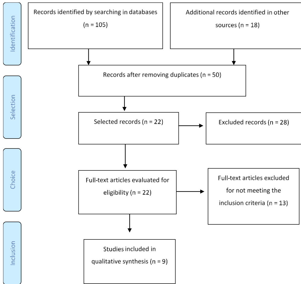
Figure 1. PRISMA flowchart
