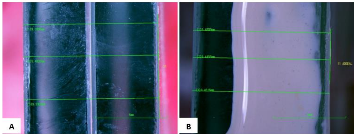
Figure 4. A. Prior thickness measurement of glass plates through stereomicroscope. B. Thickness measurement after loading 150 N through stereomicroscope
