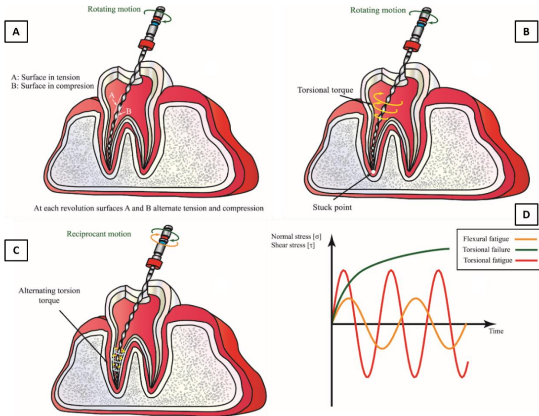
Figure 1. Failure mechanisms for NiTi endodontic files
