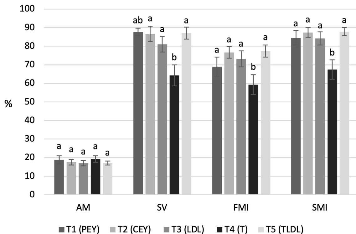
Figure 1. Morphology, vitality and membrane integrity of extended semen. AM: Abnormal Morphology. SV: Sperm Vitality. FMI: Functional Membrane Integrity. SMI: Structural Membrane Integrity. PEY: Pure Egg Yolk. CEY: Centrifuged Egg Yolk. LDL: Low-Density Lipoproteins. T: Trehalose. TLDL: Trehalose and LDL. The results are presented as mean \pm standard error of mean (S.E.M). Different letters (a, b; bars per treatment) indicate significant differences ( p < 0.05 ).
