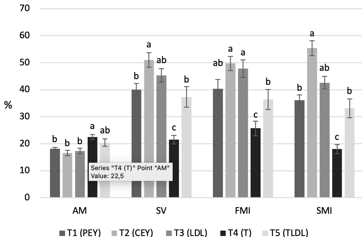
Figure 2. Morphology, vitality and membrane integrity of thawed semen. AM: Abnormal Morphology. SV: Sperm Vitality. FMI: Functional Membrane Integrity. SMI: Structural Membrane Integrity. PEY: Pure Egg Yolk. CEY: Centrifuged Egg Yolk. LDL: Low-Density Lipoproteins. T: Trehalose. TLDL: Trehalose and LDL. The results are presented as mean \pm standard error of mean (S.E.M). Different letters (a, b; bars per treatment) indicate significant differences ( p < 0.05 ).
