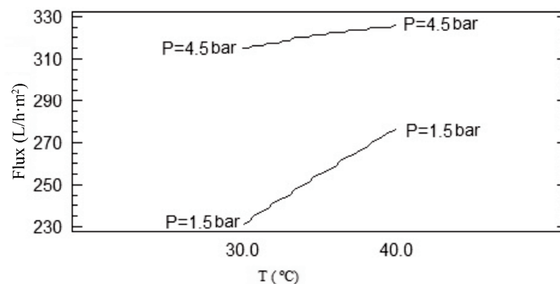
Figure 5. Interaction TMP (bar) and temperature ( ^{\circ}\text{C} ) with flux ( \text{L}/\text{h}\cdot\text{m}^2 ), obtained by means of the total recirculation method.
