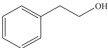
Figure 1. 2-phenylethanol (2-PE) molecular structure.
